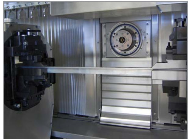
Through spindle
