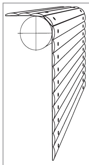
FLEXPRO (Type 4/5)
