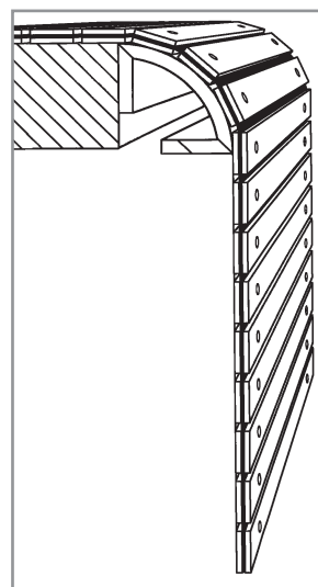
FLEXPRO (Type 1/2/3)
